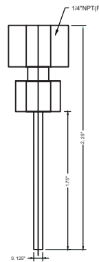
Gauge Adaptor 2.25"
