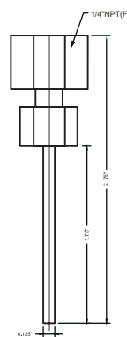
Gauge Adaptor 2.75"
